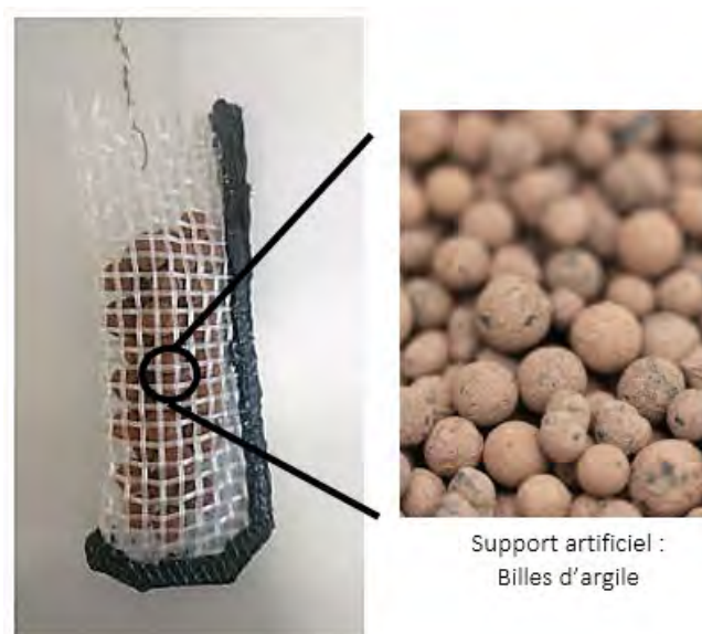
Fig. 35. Germcatcher © Photos Lehna E3S
